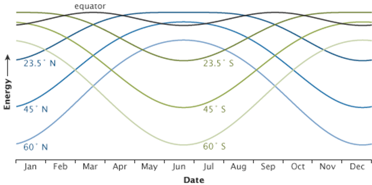
Earth's Heating Imbalances Graph | Image Credit: NASA | https://mynasadata.larc.nasa.gov/sites/default/files/inline-images/solar_insolation_date.png
