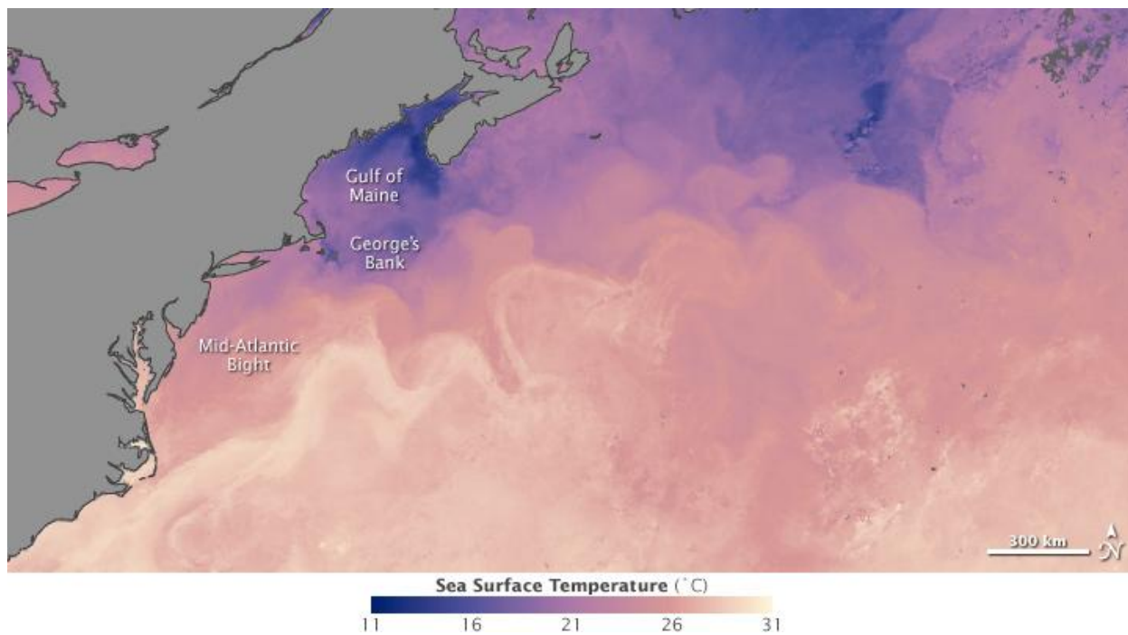
Sea Surface Temperatures (Source: NASA Earth Observatory )
