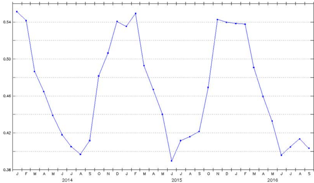
Monthly area-average albedo over Alaska: 2014-2016
