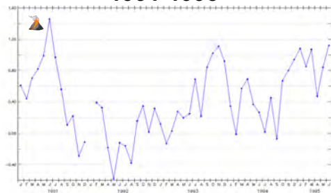
Global Mean Temperature Anomaly, 1991-1995
