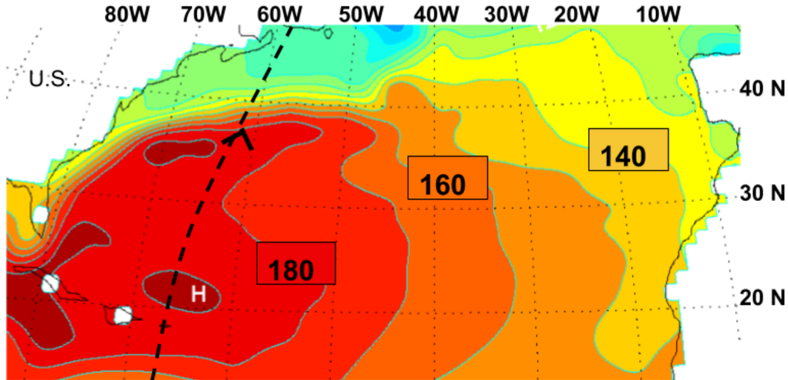
Figure 1. North Atlantic Map of Sea Surface Heights (cm)
