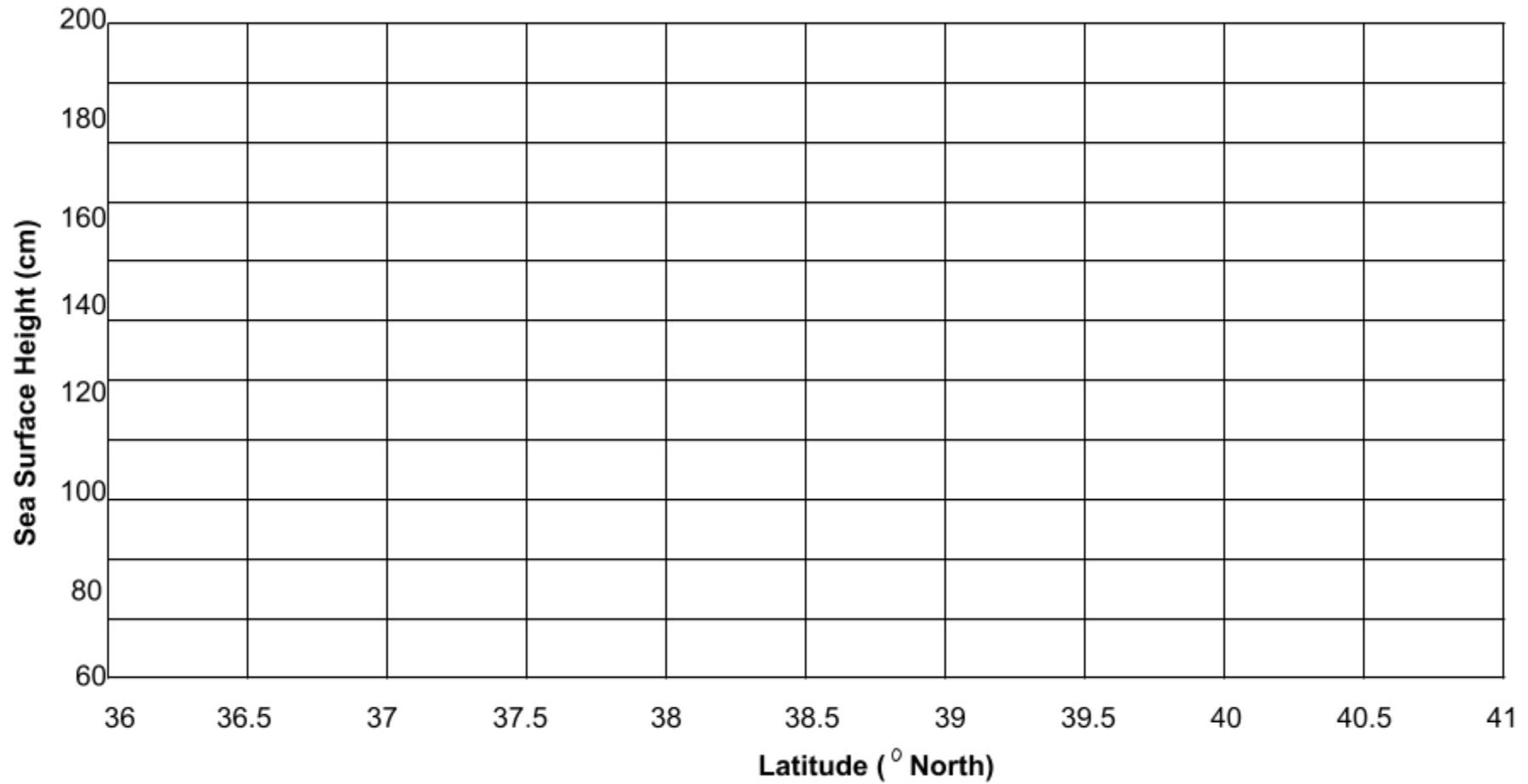
Figure 2. Sea Surface Height Plot Along Satellite Track
