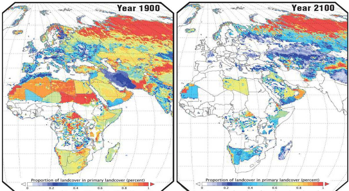
Proportion of landcover in primary landcover (percent) for 1900 and projected for 2100 Image Credit: NASA Oak Ridge National Laboratory DAAC https://mynasadata.larc.nasa.gov/sites/default/files/inline-images/primary%20land%20cover_0.jpg
